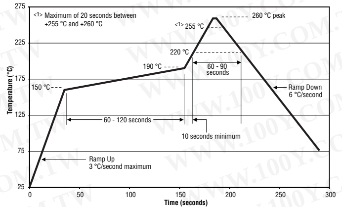
Soldering Profile
